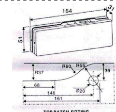
TOP PATCH FITTING
