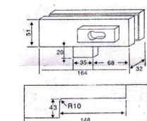
BOTTOM OR TOP PATCH LOCK FITTING WITH 22mm BOLT THROW AND SECURITY PROFILE SOLUTION
