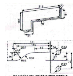
TO SIDE PANEL PIVOT PATCH FITTING
