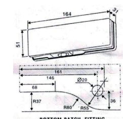
BOTTOM PATCH FITTING
